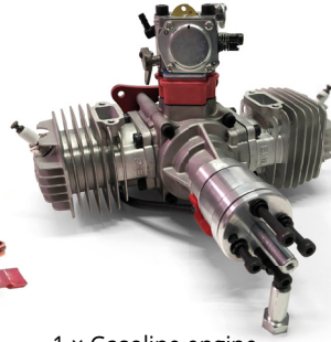
1 × Gasoline engine EME 70 cm³ Boxer
