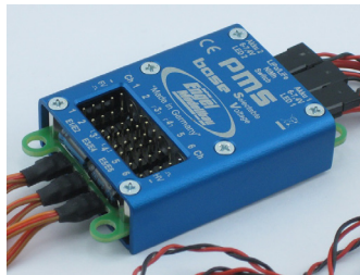
1 × Power Management System „Base“ SV Akkuweiche
