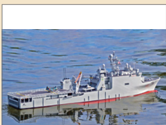
E 22 US-Dockschiiff LSD-44 Gunston Hall von Dirk Lübbesmeyer
